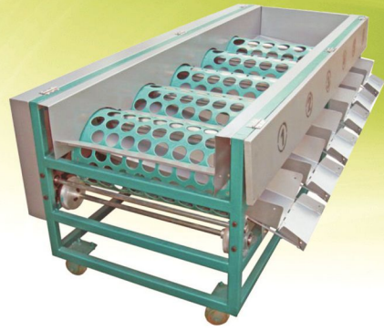
Fruit Grading Machine
