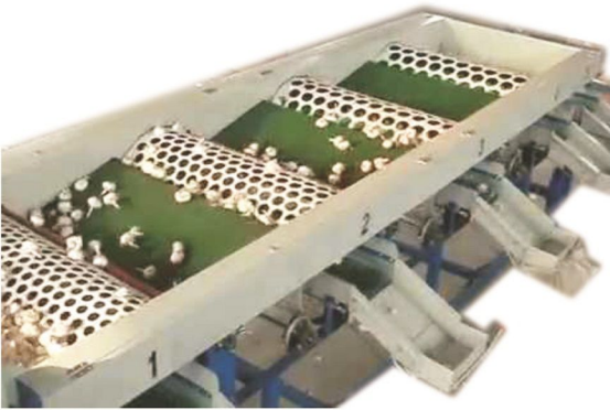
Grading Machine
