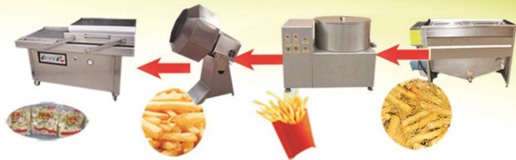
French Fry Plant
